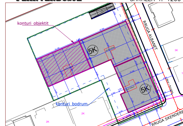
SHKALLA 1: 1200
